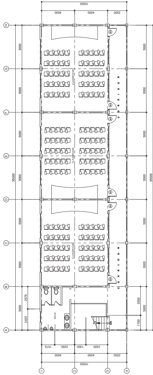
TYPICAL 2ND AND 3RD FLOOR PLAN
