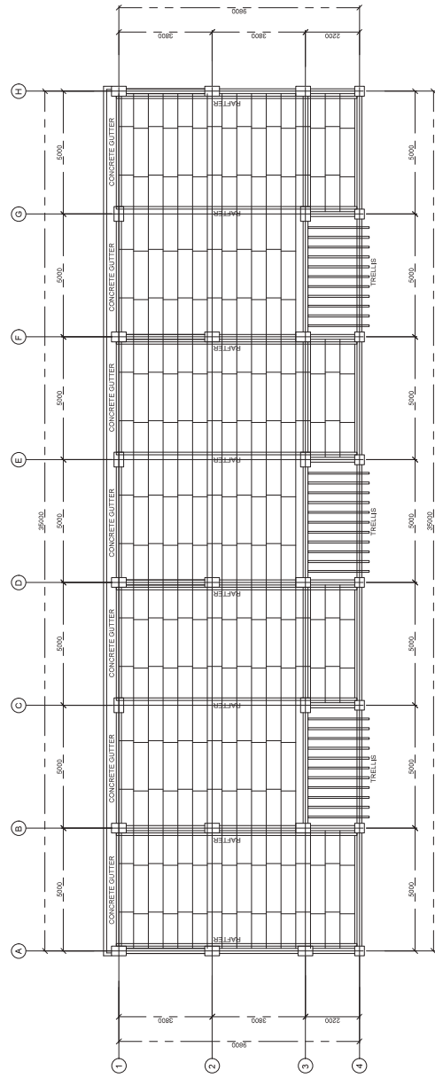
2 ROOF FRAMING PLAN 1:1000
