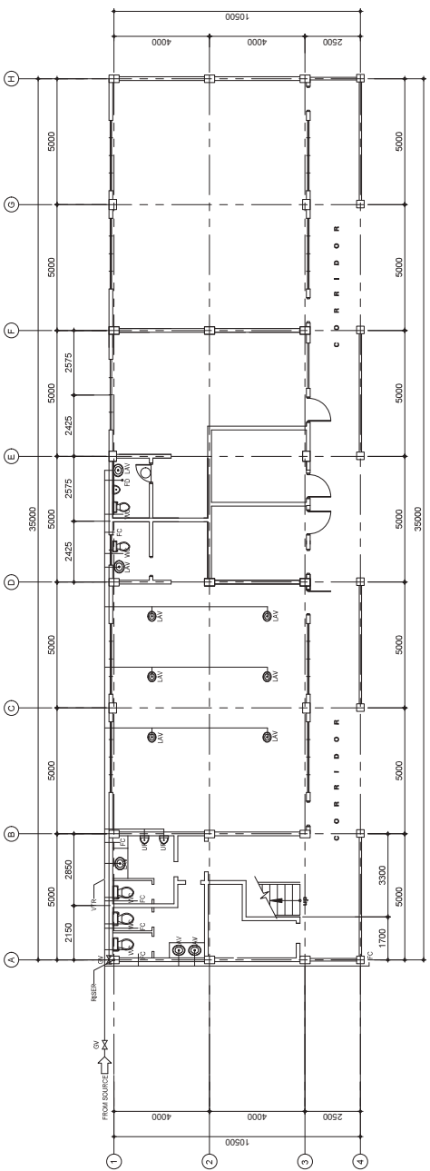
1 GROUND FLOOR WATER LAYOUT
