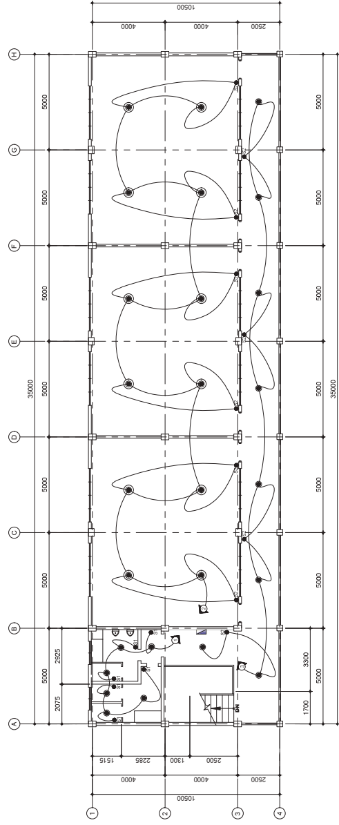
2. TYPICAL 2ND AND 3RD FLOOR LIGHTING LAYOUT
