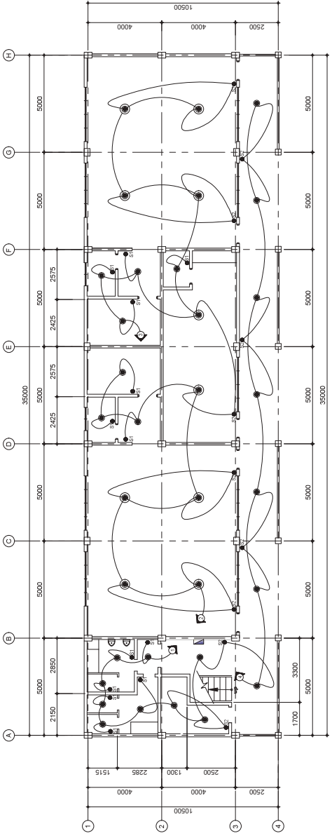
1. GROUND FLOOR LIGHTING LAYOUT
