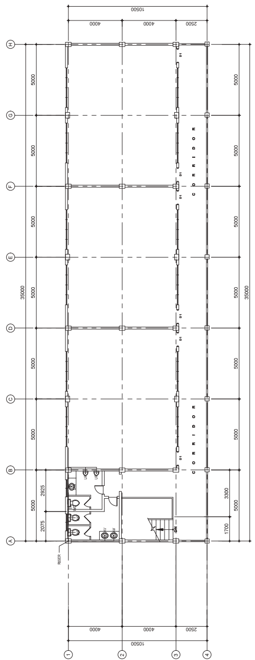
2 TYPICAL 2ND AND 3RD FLOOR WATER LAYOUT
