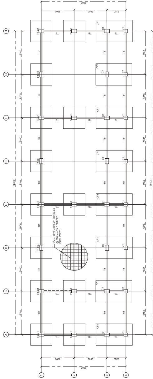
1. FOUNDATION PLAN
