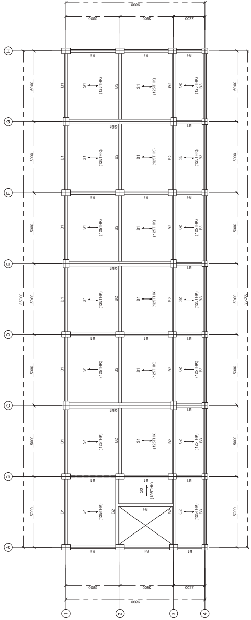
2. 2ND AND 3RD FLOOR FRAMING PLAN
