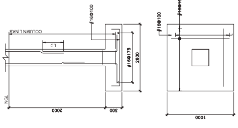
3. F2-C2 DETAIL
