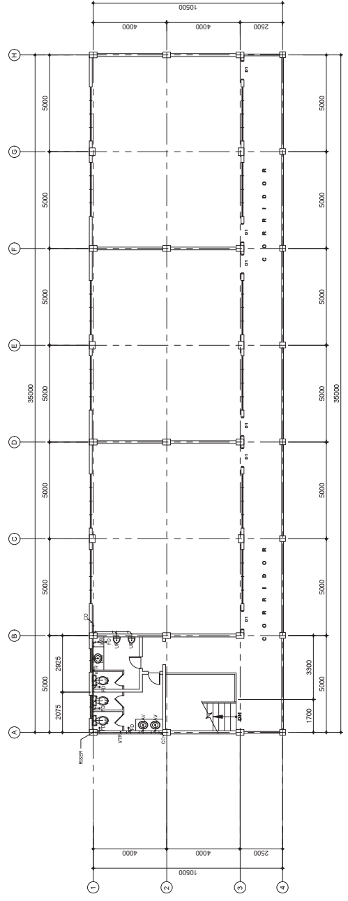
2. TYPICAL 2ND AND 3RD FLOOR PLUMBING LAYOUT
